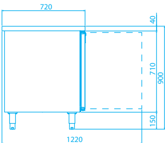
Tampo superior central
